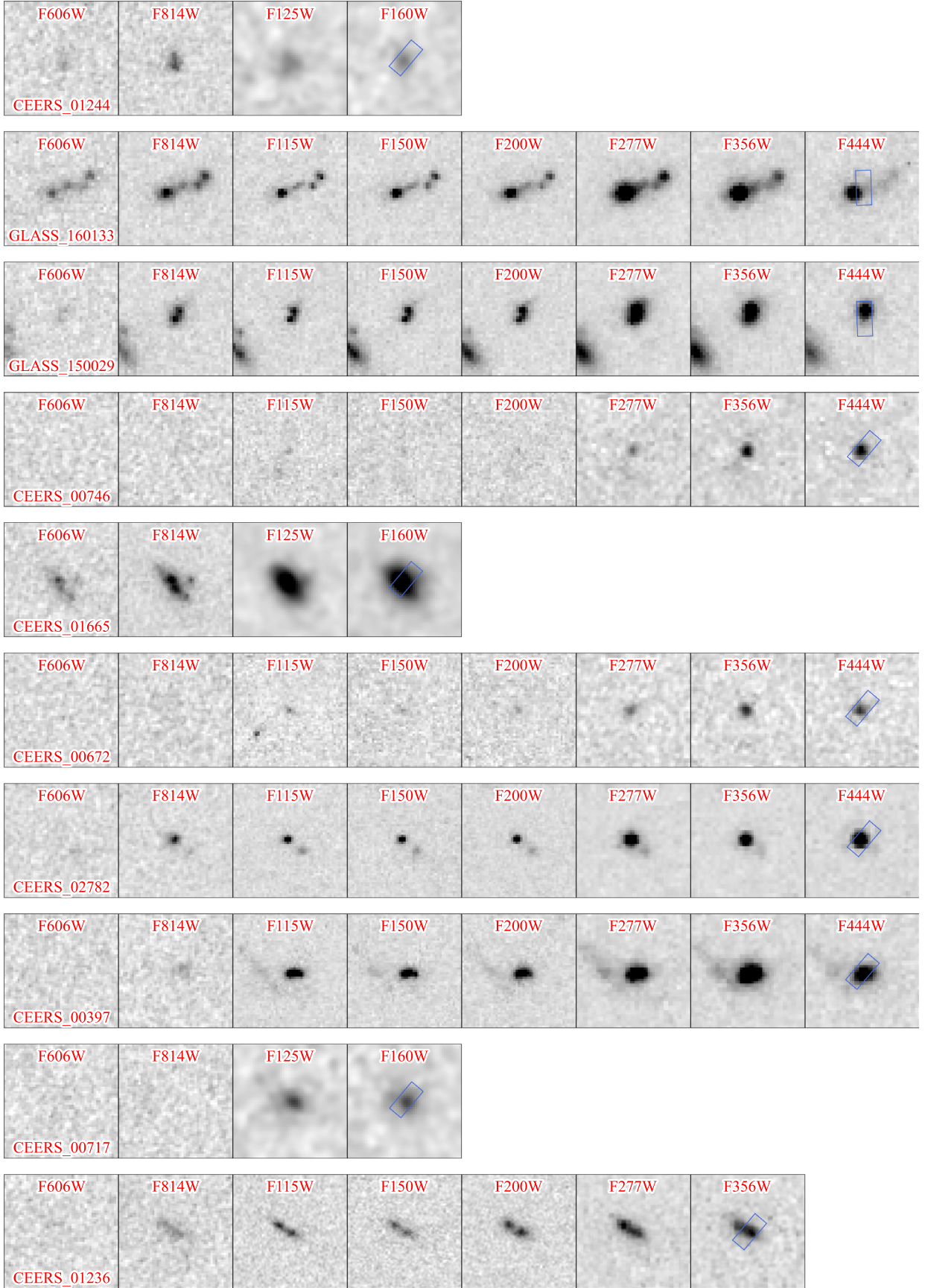
Figure 5. 3'' × 3'' images of our faint type 1 AGNs. The HST/ACS F606W, F814W, and the JWST/NIRCam F115W, F150W, F200W, F277W, F356W, and F444W images are shown. For objects whose NIRC images are not available, we instead show the HST/WFC3 F125W and F160W images. The NIRSpec MSA aperture is shown with the blue rectangle in the longest wavelength band. More than half of the sources show extended morphologies, indicating that the total lights are significantly contributed by their host galaxies.
